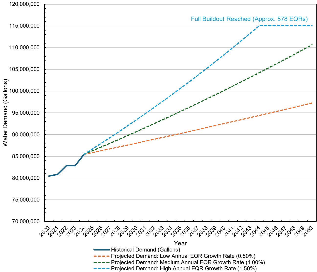
Figure 6 Historical and Projected Annual Water Demands City of Creede
